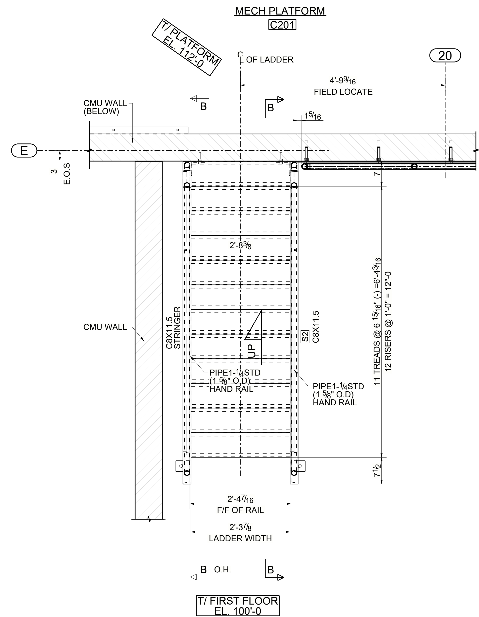
SHIP LADDER PLAN @ AREA-C MECH PLATFORM-C201 @ FIRST FLOOR EL.100'-0" (REFER : PLATFORM-AREA-C/A-151B & S-151C )
