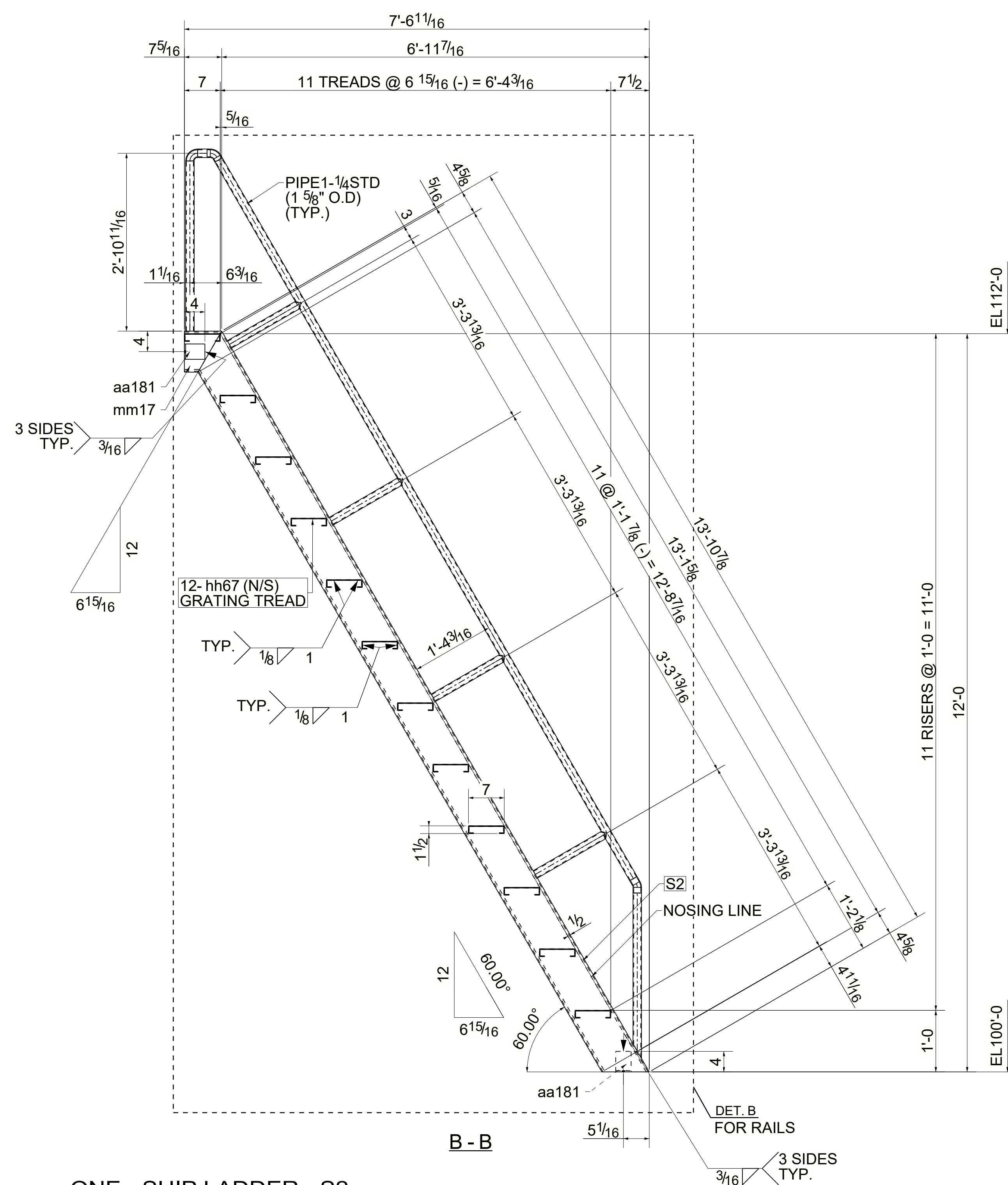
ONE - SHIP LADDER - S2
