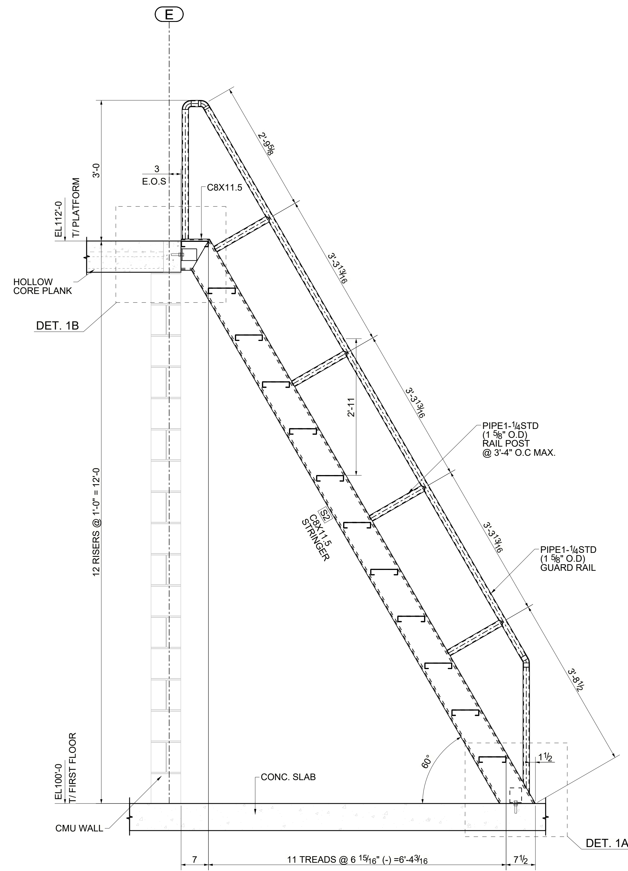
SECTION B - B (REFER : TYPICAL SHIPS LADDER DETAIL @ PLATFORM-C/A-151B)
